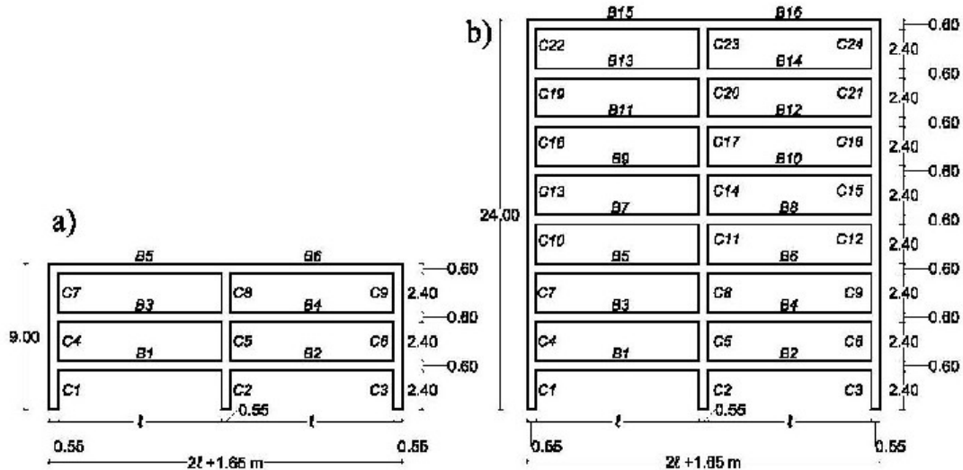
Fig. 3 – (a,b) A three and eight storied building frame, where l (m) is the clear beam span. There are two sets of buildings. One with l=10.0 (m) and another with l=4.0 (m). The alphanumeric indicators show the column (C) or beam (B) number, to which the comparison of the developed member forces is carried out (see Figs 4,5,6,7).
