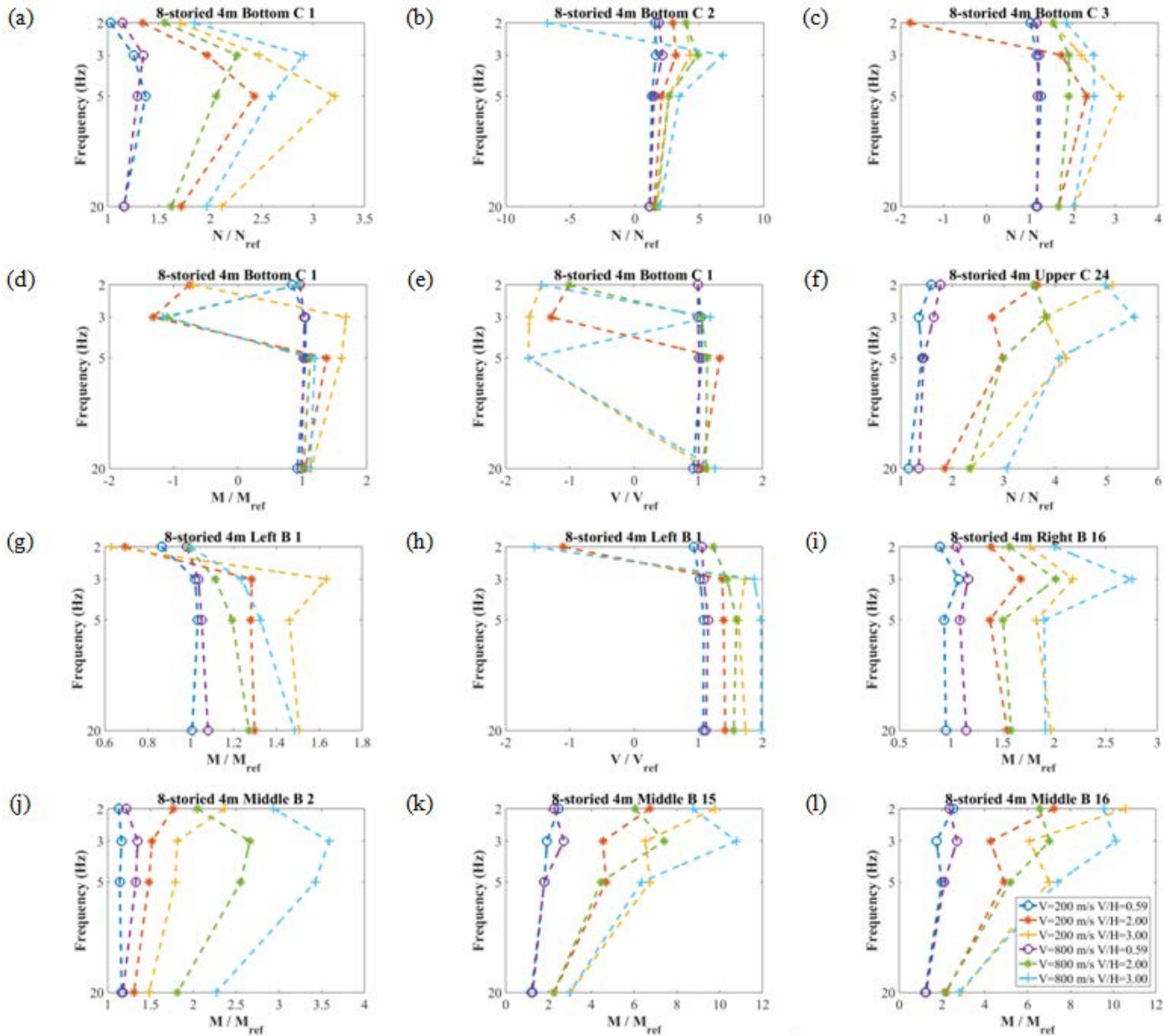
Fig. 7 – Ratios of Axial Forces (N) over ( N_{ref} ), Moments (M) over ( M_{ref} ) and Shear Forces (V) over ( V_{ref} ), developed at various locations of the eight storied building frame, with a clear beam span of 4.0 (m). The key alphanumeric indices indicate the location of the column (C) or beam (B) cross section, and they are respectively shown in Fig. 3.
