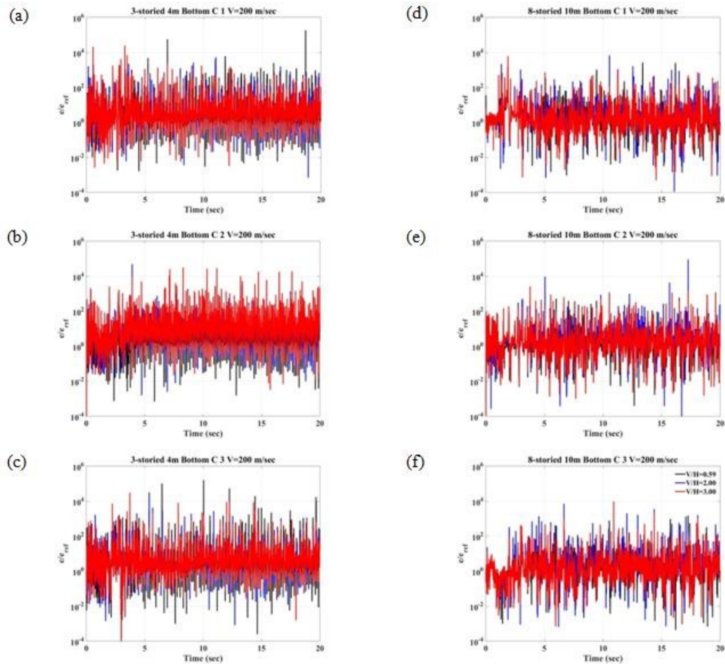
Fig. 8 – Ratios of the eccentricities e/e_{ref}=(M/N)/(M_{ref}/N_{ref}) at the bottom of the three lower columns during the whole time of analysis. (a), (b), (c) Three storied building frame with 4.0 (m) clear beam span, and (d), (e), (f) eight storied building frame with 10.0 (m) clear beam span.
