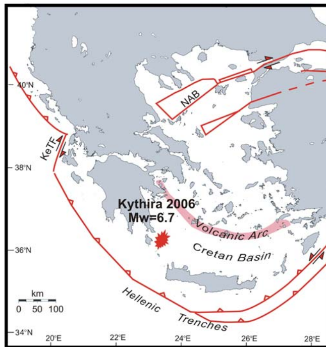
Figure 1. On January 8, 2006 a M_w=6.7 thrust faulting event occurred on the Hellenic subduction zone. The epicentre was located about 30 km east of the island of Kythira and the focal depth was estimated at 70 km.
