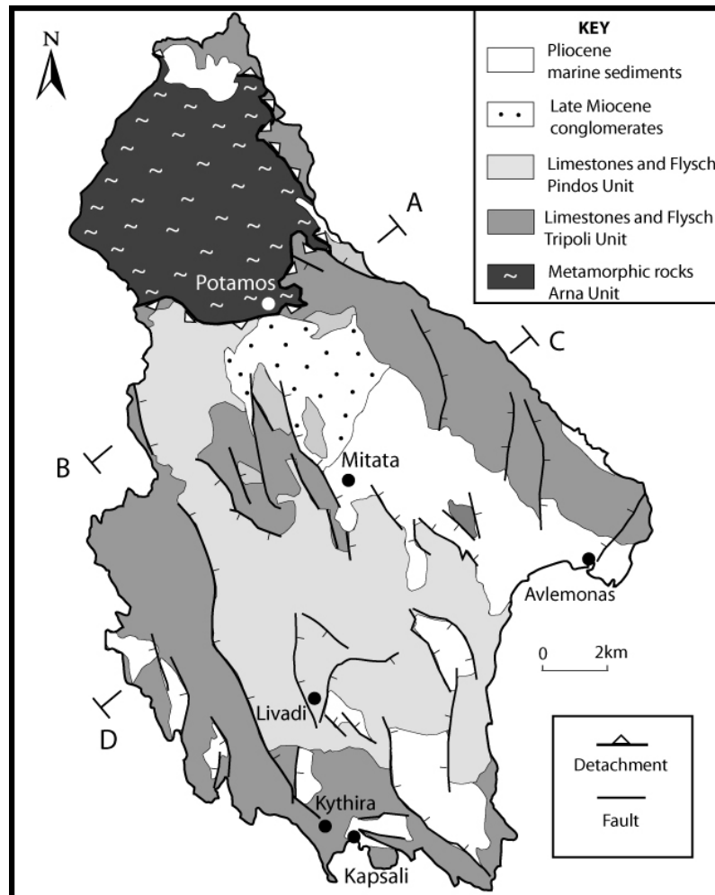
Figure 5. Geological map of the Kythira island (modified from PAPANIKOLAOU AND DANAMOS 1991). Letters A, B and C, D show the traces of the cross sections presented in Figure 6.
