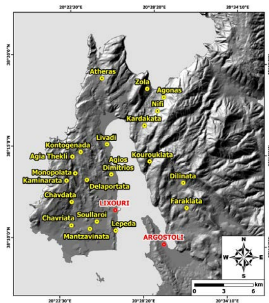
Fig. 5 – Locations of Lixouri and Argostoli towns and villages in the Paliki peninsula that suffered damage by both earthquakes.
