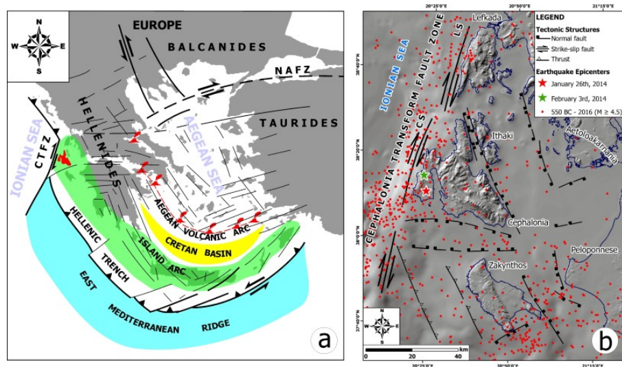
Fig. 1 – (a) Structural sketch of the Hellenic Arc showing the location of the Cephalonia Island at the northwesternmost part of the Hellenic Arc [6, 7]. (b) The central part of the Ionian Islands controlled by the Cephalonia Transform Fault Zone (CTFZ) comprising the Cephalonia segment (CS) and the Lefkada segment (LS). The epicenters of the early 2014 Cephalonia earthquakes (January 26 and February 3) and the epicenters of earthquakes with magnitude \geq 4.5 for the period extending from 550 BC to April 2, 2016 [8] are also shown.
